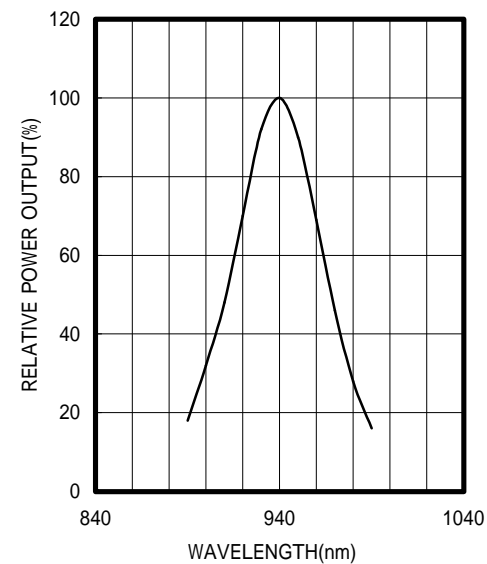
SPECTRAL OUTPUT
