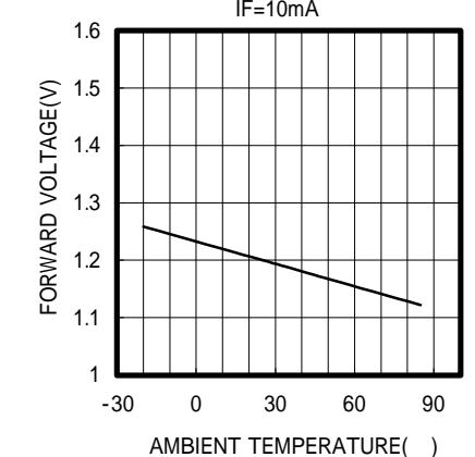
FORWARD VOLTAGE vs TEMPERATURE IF=10mA
