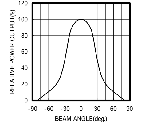
RADIATION PATTERN
