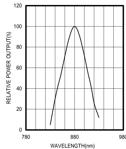
SPECTRAL OUTPUT
