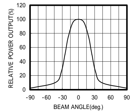
RADIATION PATTERN
