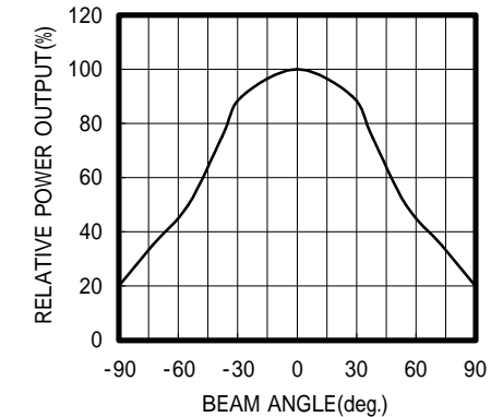
RADIATION PATTERN
