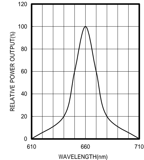
SPECTRAL OUTPUT
