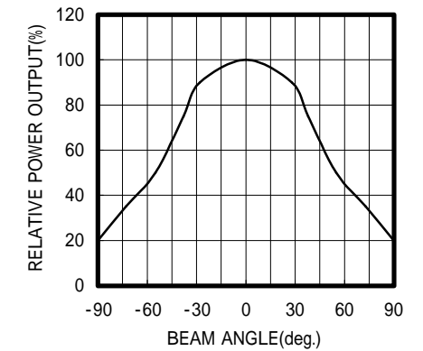
RADIATION PATTERN
