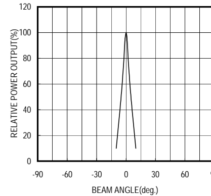
RADIATION PATTERN
